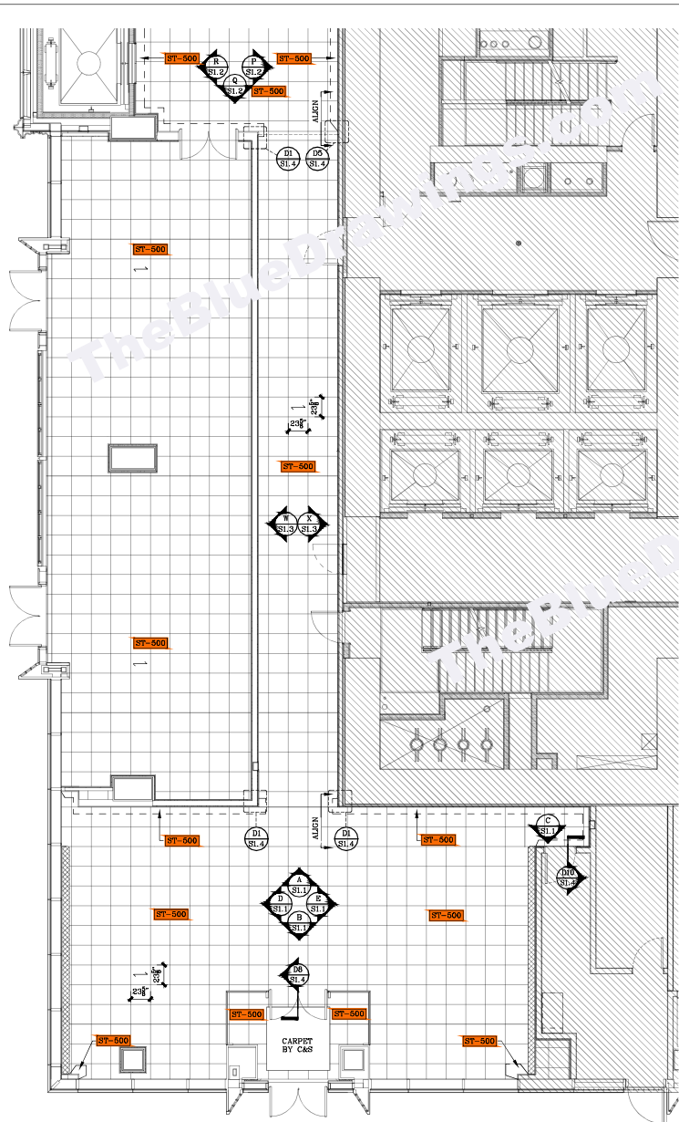
2 PLAN @ LEVEL 1B SCALE: 3/16"=1'-0"
