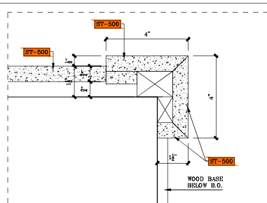
③ PLAN DETAIL SCALE: 6"=1'-0"
