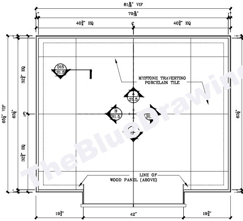
1 PLAN @ ELEVATOR CAB SCALE: 1"=1'-0"
